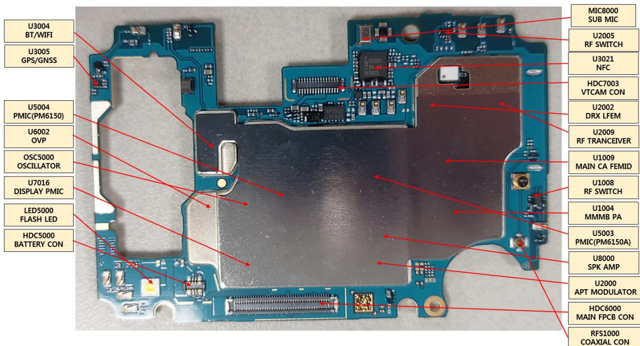
MAIN PBA (BOTTOM SIDE)
